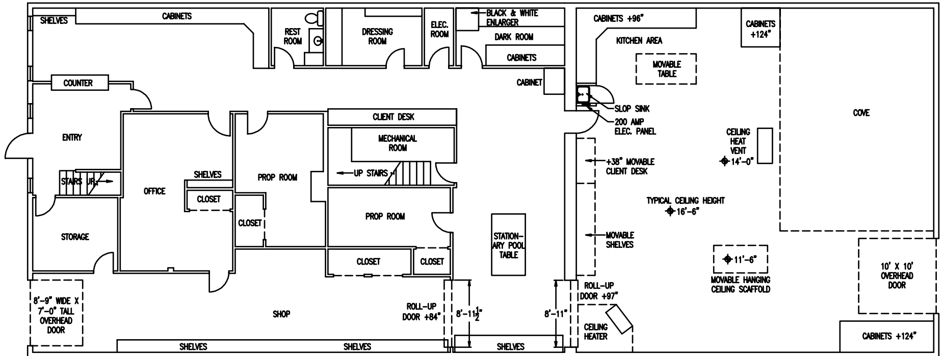
← N STUDIO FLOOR PLAN NO SCALE
